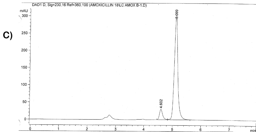
Supplementary Figures S1. HPLC peaks for amoxicillin: A) standard antibiotic load 10 ppm (2.0 ng/ul); B) intracellular antibiotic in E. coli cells treated with the antibiotic and FS-1; C) intracellular antibiotic in E. coli cells treated with the antibiotic only. Axis X depicts elution minutes; axis Y - milli-Absorbance Units (mAU).
