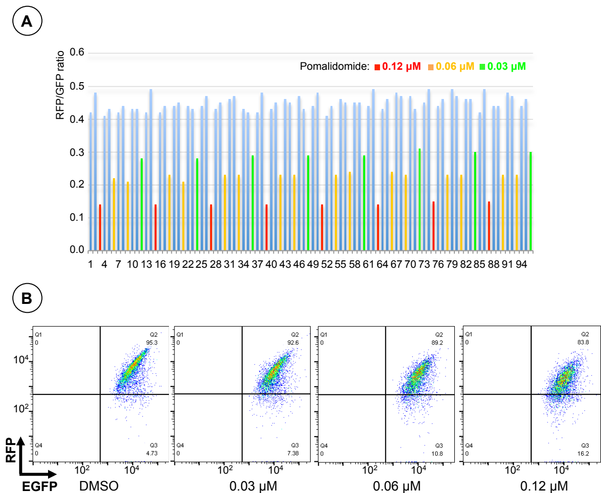
Supplementary Figure 3: Effect of pomalidomide on IKZF3 stability. SFFV-GP-IKZF3R cells were seeded in a 96 well plate. A: Pomalidomide was added 16 h before collecting cells at 0.03 (green), 0.06 (yellow) and 0.12 (red) \mu M. DMSO was added in the other wells. The mean of the ratios of RFP to EGFP fluorescence intensities are represented for each well. A clear and reproducible dose-dependent decrease in the amount of IKZF3-RFP was visible. B: examples of the FlowJo plots of RFP and EGFP fluorescences for control (well 11) and the three pomalidomide concentrations (wells 3, 9 and 12).
