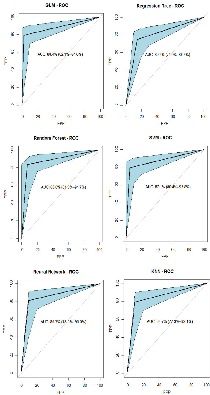
S6: Composite AUC-ROC curves
